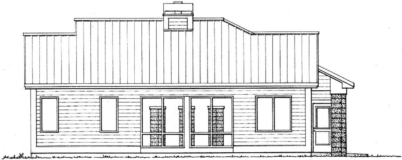
SOUTH ELEVATION
