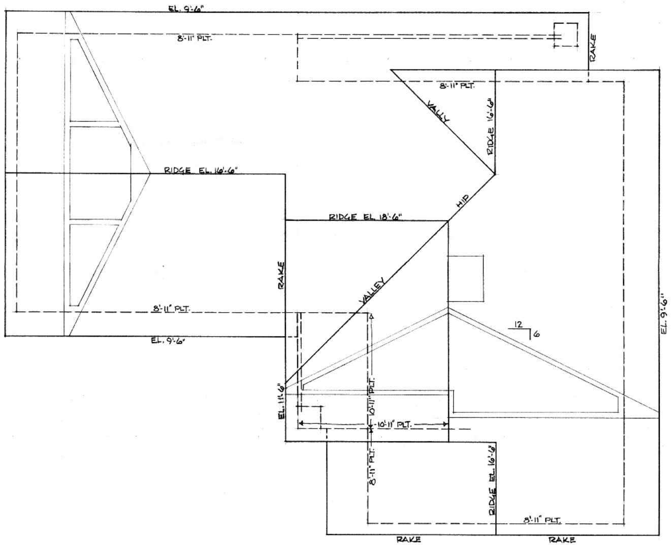
ROOF PLAN
